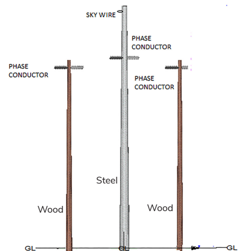
Proposed three-pole wood and steel structure
