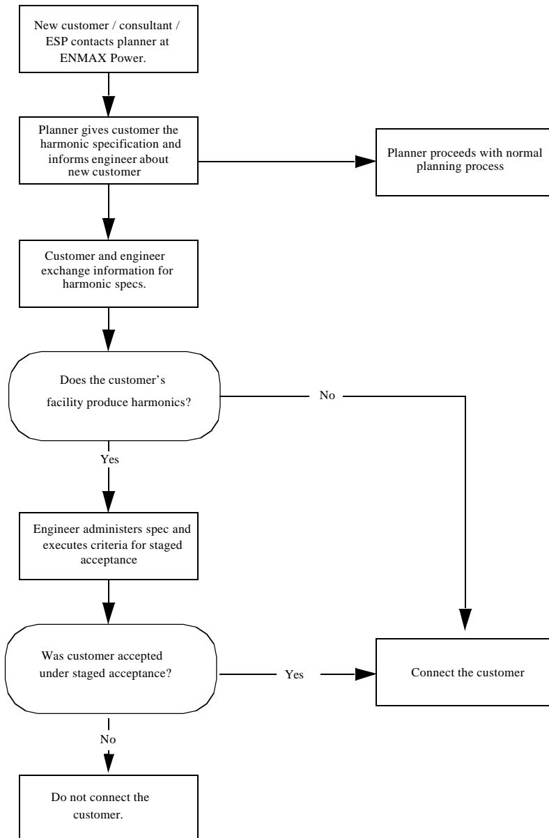
Figure 3.2 Commissioning Process
